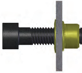
STANDARD RIVET NUT INSTALLED
