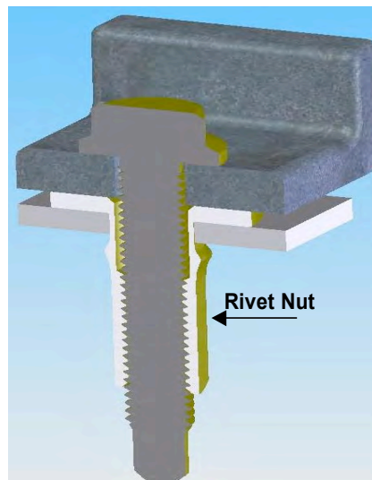
Agricultural – High Strength Rivet Nut
