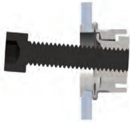
CROSS SECTION OF RIV-FLOAT®-SHORT Installed
