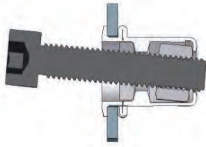
CROSS SECTION OF RIV-FLOAT® INSTALLED
