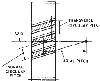
FIGURE 1.10 — NORMAL, TRANSVERSE & AXIAL PITCH
