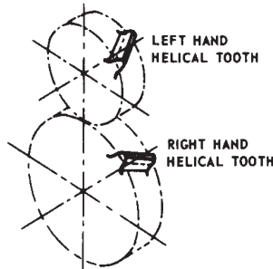
FIGURE 1.3 — PARALLEL HELICAL GEARS
