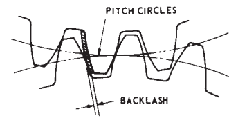
FIGURE 1.12 — BACKLASH
