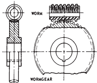
FIGURE 1.2 — WORMGEARING
