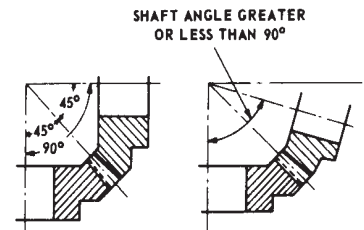
FIGURE 1.5b — MITER GEARS
