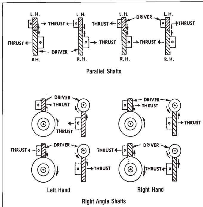
FIGURE 2.4 — THRUST LOADING DETAILS
