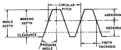
FIGURE 2.1 — BASIC RACK — (NORMAL PLANE)
