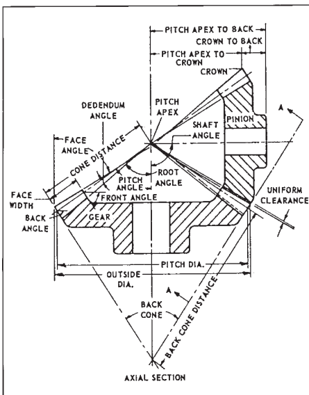
FIGURE 2.5 — BEVEL GEAR NOMENCLATURE
