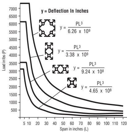
Fixed at both ends, load at center
