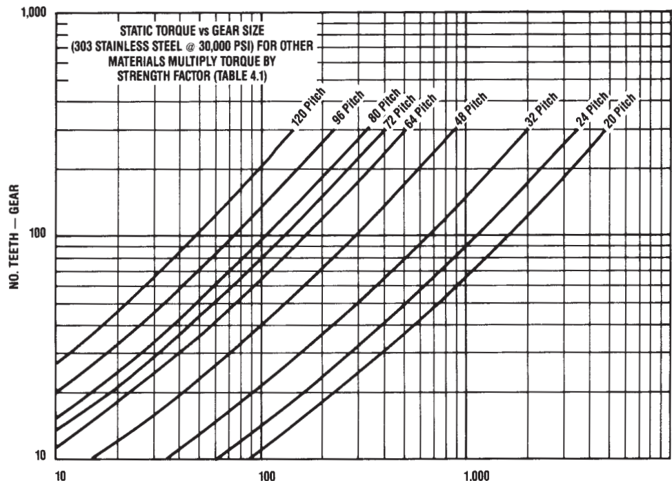
FIGURE 4.1 — STATIC TORQUE IN. OZ. (PER 1/16" FACE WIDTH GEAR)
