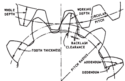
FIGURE 2.2 — SPUR, HELICAL, GEAR NOMENCLATURE
