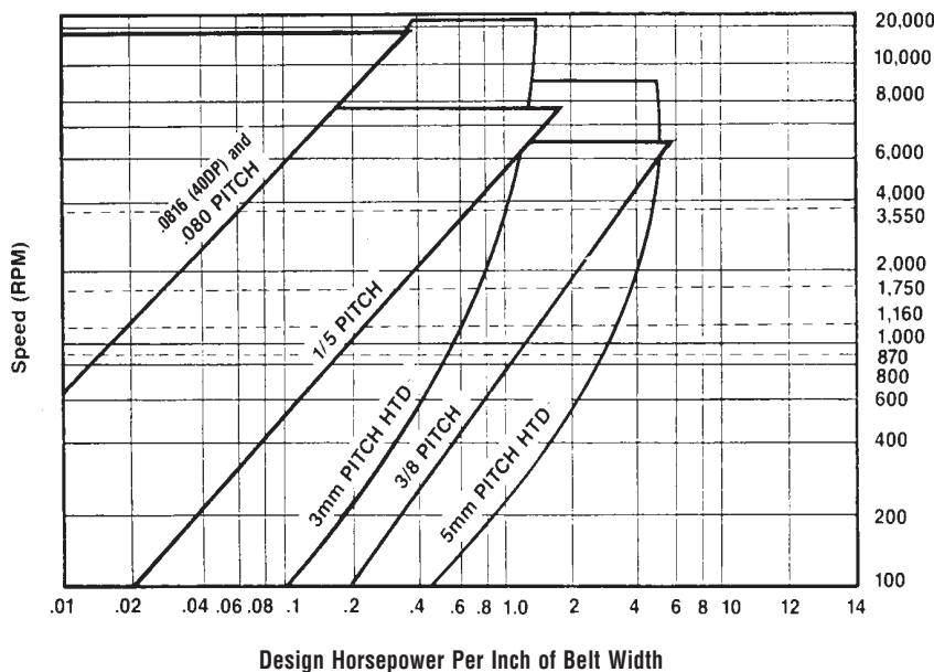
E*P*S Drive Selection Chart
