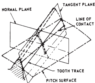
FIGURE 1.8 — NORMAL & TANGENT PLANES
