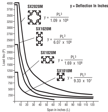
Fixed at both ends, load at center
