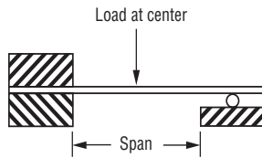
Fixed at one end, sliding at one end, load at center
