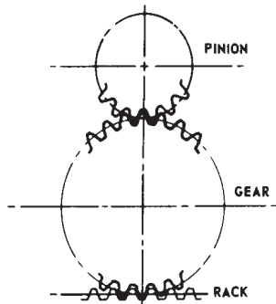
FIGURE 1.1 — GEARS
