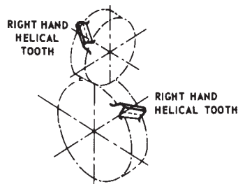
FIGURE 1.4 — CROSSED HELICAL GEARS
