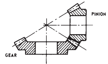
FIGURE 1.5a — BEVEL GEARS
