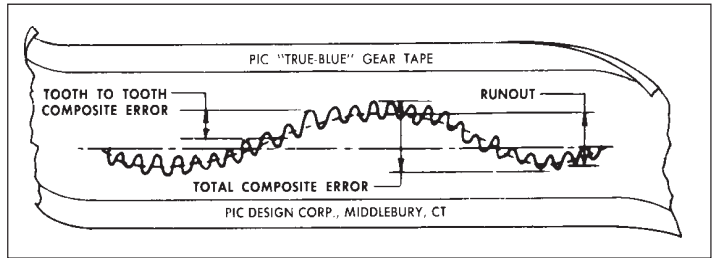
FIGURE 5.1 — "TRUE BLUE" GEAR TAPE
