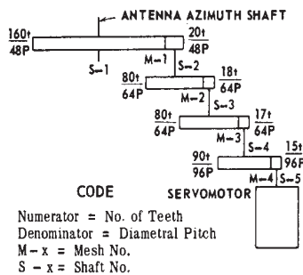
FIGURE 3.1 — GEARING SCHEMATIC AND DESIGN DETAILS FOR A SMALL RADAR ANTENNA DRIVE GEAR TRAIN
