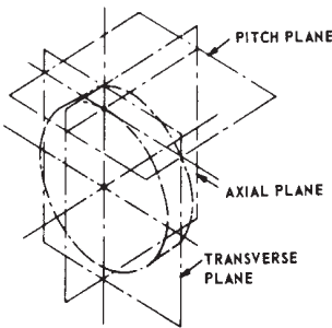
FIGURE 1.7 — PITCH, AXIAL & TRANSVERSE PLANES
