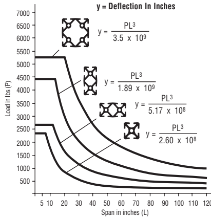
Fixed at one end, sliding at one end, load at center
