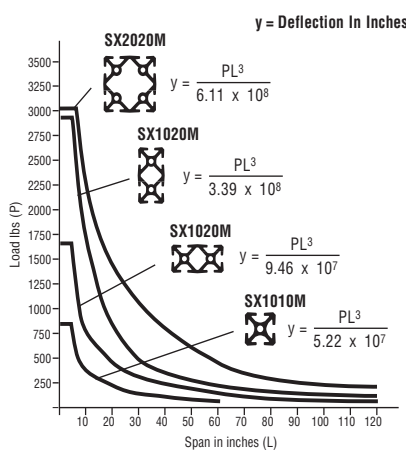
Fixed at one end, sliding at one end, load at center
