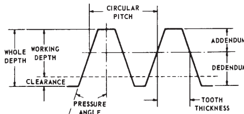
FIGURE 1.11 — BASIC RACK (NORMAL PLANE)
