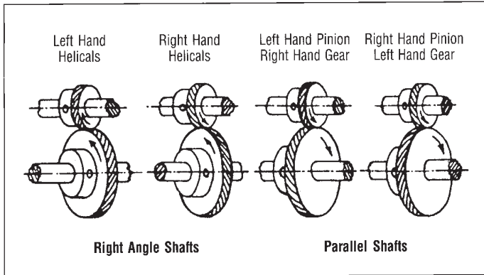
FIGURE 2.3 — HELICAL GEARS OF THE SAME HAND MESH AT RIGHT ANGLES — HELICAL GEARS OF THE OPPOSITE HAND MESH ON PARALLEL SHAFTS
