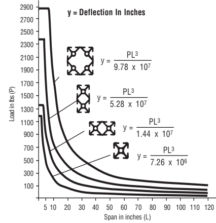
Fixed at one end, load at unsupported end
