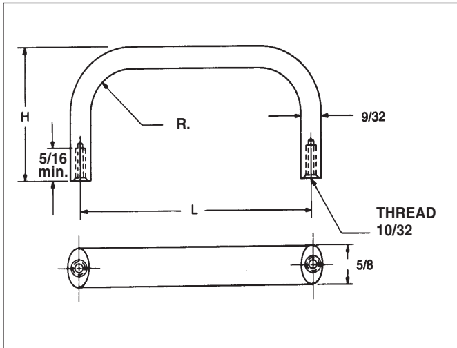
5/8 x 9/32 Oval Internal Thread Handle Aluminum — Black Anodize (10-32 Thread)
