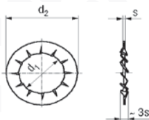
DIN 6798 Type J Internally Toothed
