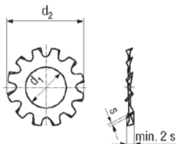
DIN 6797 Type A Externally Toothed
