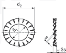
DIN 6798 Type A Externally Toothed
