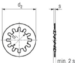
DIN 6797 Type J Internally Toothed
