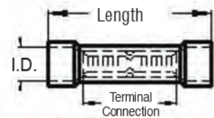
Molded Nylon Insulated Seamless or Butted Seam Butt Connector
