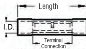
Extruded Nylon Insulated Seamless or Butted Seam Butt Connector
