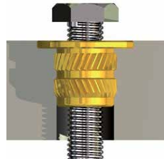
Typical Flange Installation
