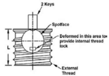
Self-Locking
