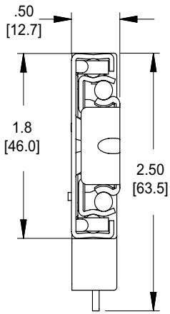
38EL Slide with Electronic Lock 100 lbs./pr. [50 kg]
