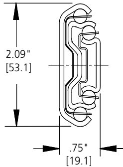
3601 255 lbs./pr. [116 kg] 3600/3607/3657 273 lbs./pr. [124 kg]
