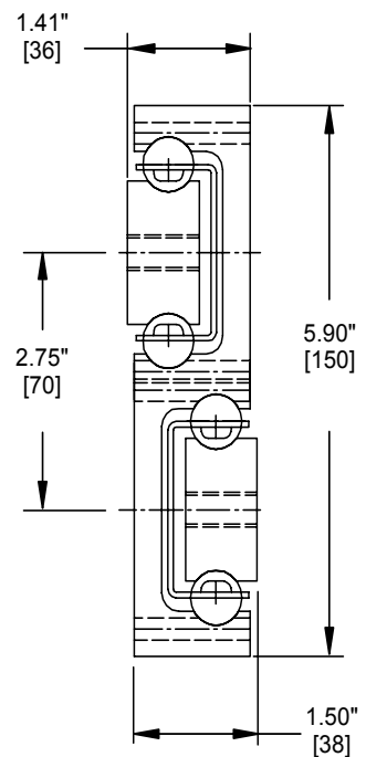
AL4140 Up to 1,323 lbs./pr. [600 kg]
