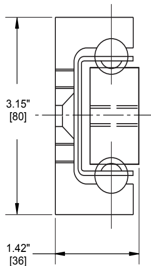
AL4120 Up to 1,212 lbs./pr. [550 kg]
