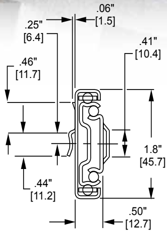
3820 Up to 100 lbs./pr. [50 kg]
