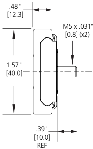
115RC Up to 265 lbs. [120 kg]
