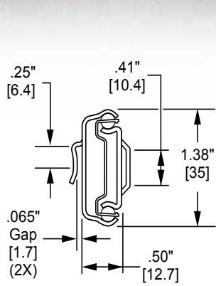
2120 Up to 75 lbs./pr. [50 kg]
