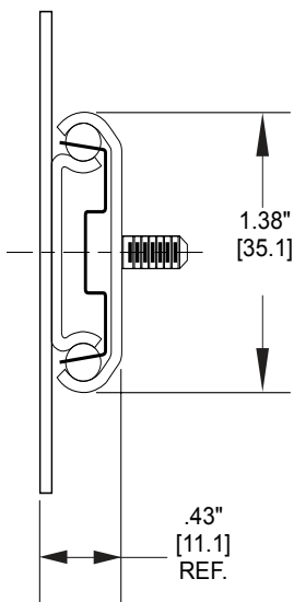
115 Side Mount: 100 lbs./pr. [50 kg] Fl.
