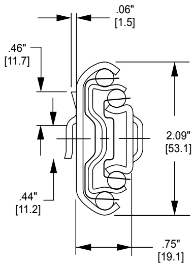
3620 Up to 200 lbs./pr. [91 kg]
