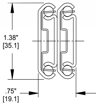
305A-LR 140 lbs./pr. [64 kg]
