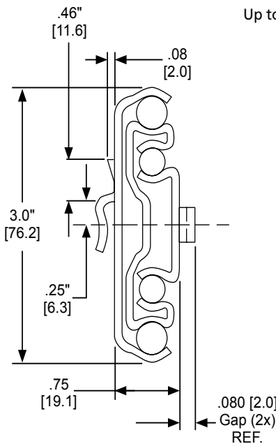
9328/9322 Up to 300 lbs./pr. [136 kg]* * depending on usage
